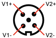
M12 DC power cable pin assignment & wire code
